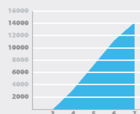
Annual kWh at mean wind speed (m/s)
